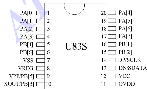
20-pin AT8PU83S D-Type PDIP/SOP
