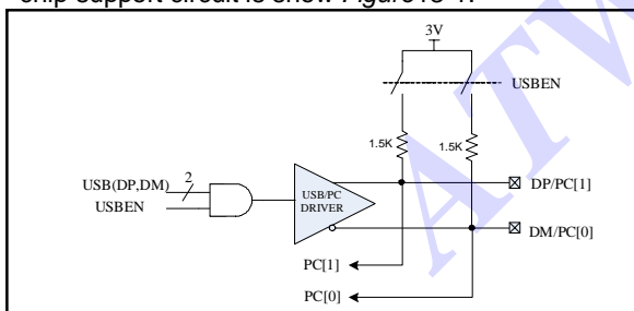
Figure13-1 Block diagram of USB Driver
